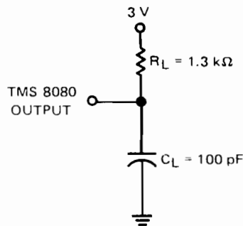
LOAD CIRCUIT
