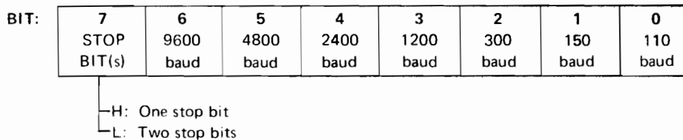
FIGURE 5—DATA BUS ASSIGNMENTS FOR RATE COMMANDS
