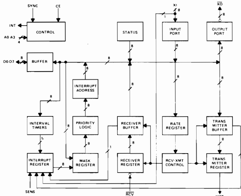
FIGURE 1—TMS 5501 BLOCK DIAGRAM
