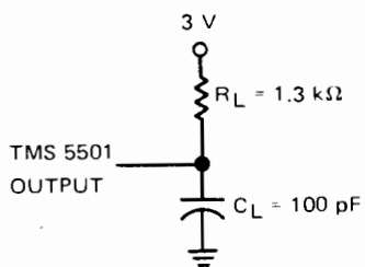
LOAD CIRCUIT
