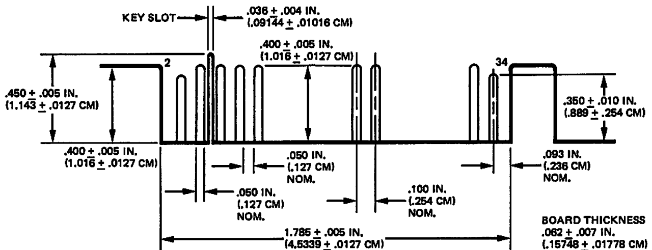
Figure 2-4. J1 Connector Dimensions
