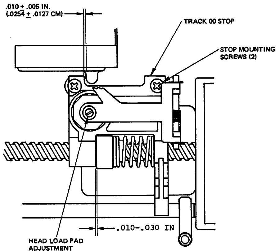
Figure 5-2. Track 00/39 Stop and Head-Load Pad Adjustment
