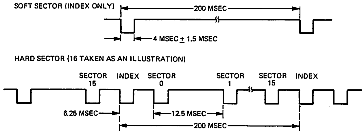
Figure 2-9. Index/Sector Timing
