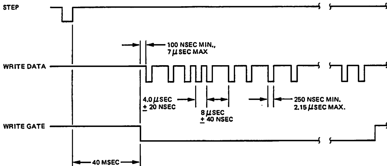
Figure 2-10. Write Timing
