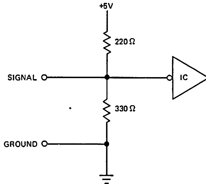
Figure 2-6. Termination Configuration
